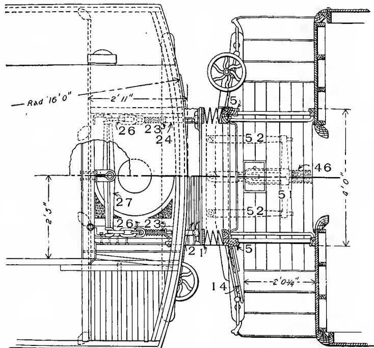
Fig. 2443. Section Plan, showing Equalizers and Springs for the Adjustment of Face-plates.
